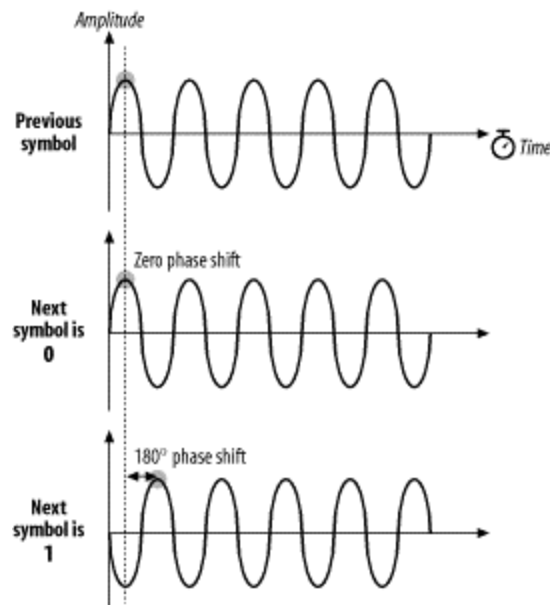
Figure 10-19. DBPSK encoding
