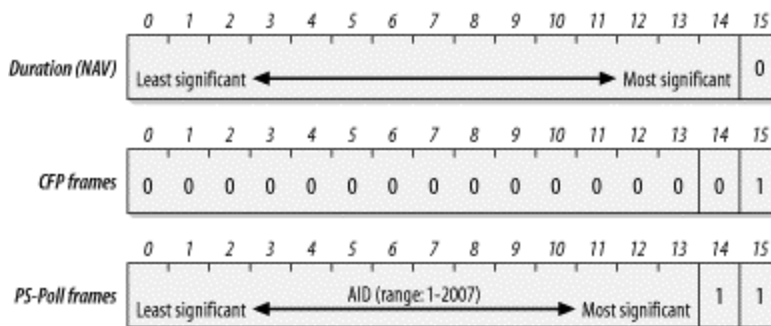
Figure 3-11. Duration/ID field
