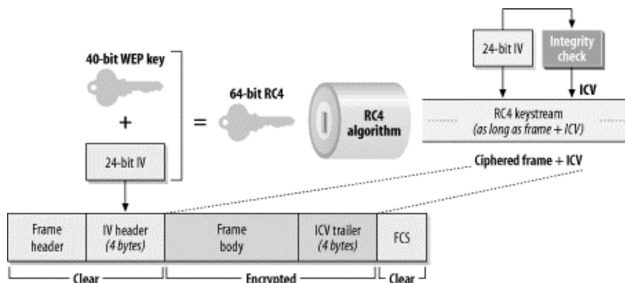
Figure 5-3. WEP operations
