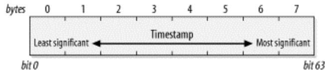
Figure 4-28. Timestamp field
