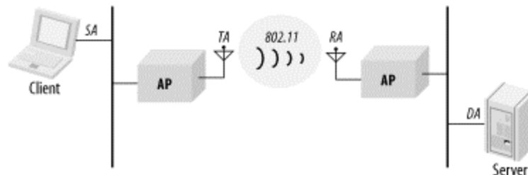
Figure 4-6. Wireless distribution system
